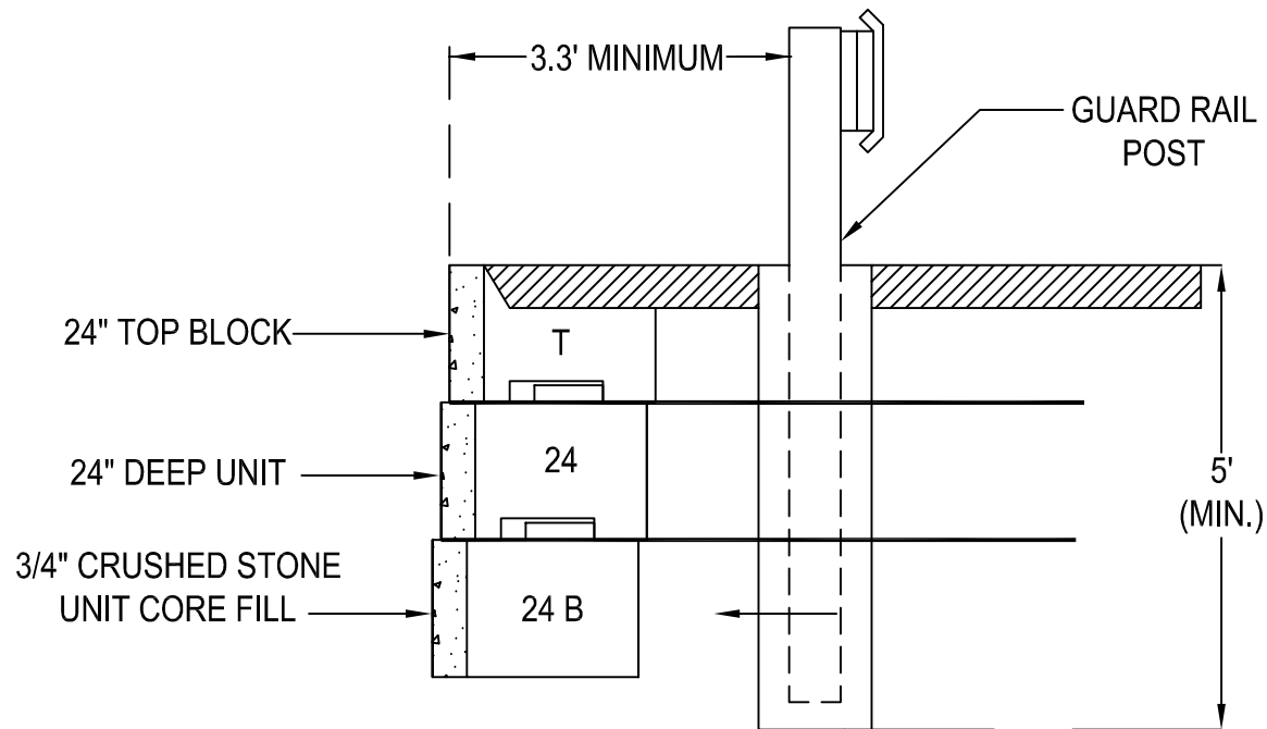
GUARD RAIL DETAIL NOT TO SCALE
