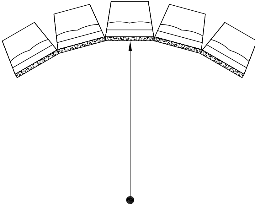
MINIMUM CONCAVE / INSIDE RADIUS FOR FULL BLOCK
