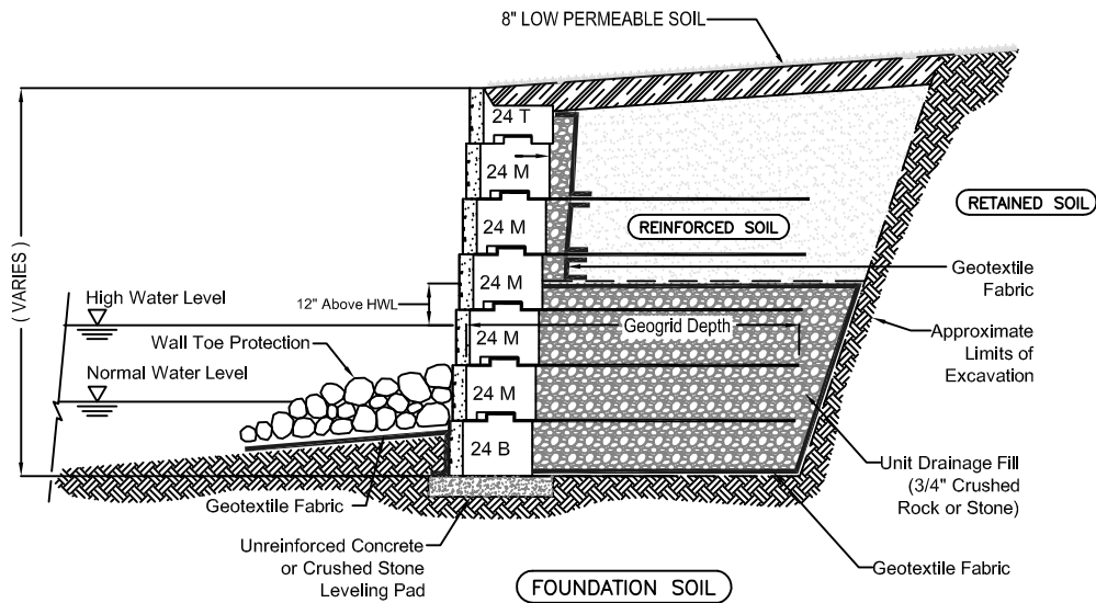
Typical Reinforced Water Wall Section
