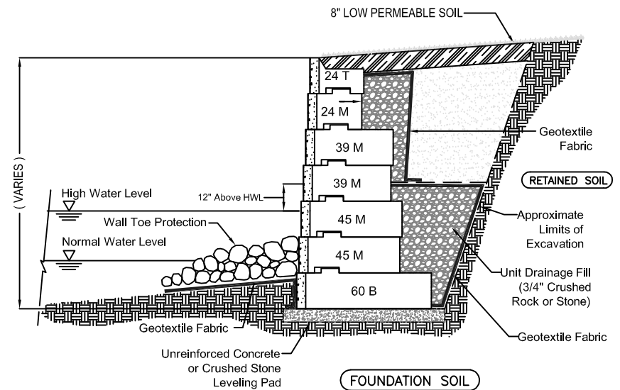
Typical Gravity Water Wall Section
