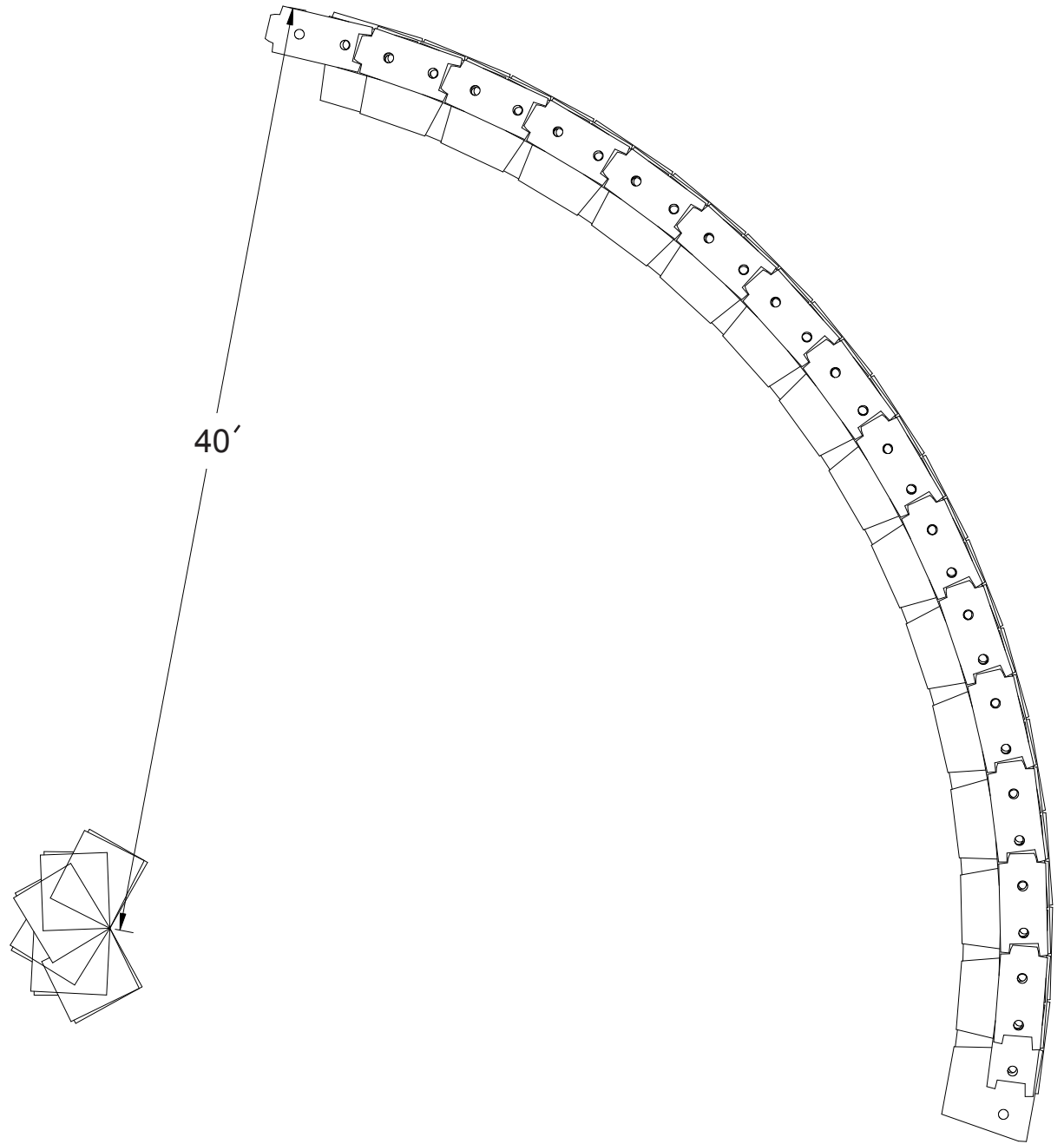
ReCon Guardrail Block Minimum Turning Radius, Outside Curve 40' Radius with 2" cut/removed from inside wing of Guardrail Block in field
