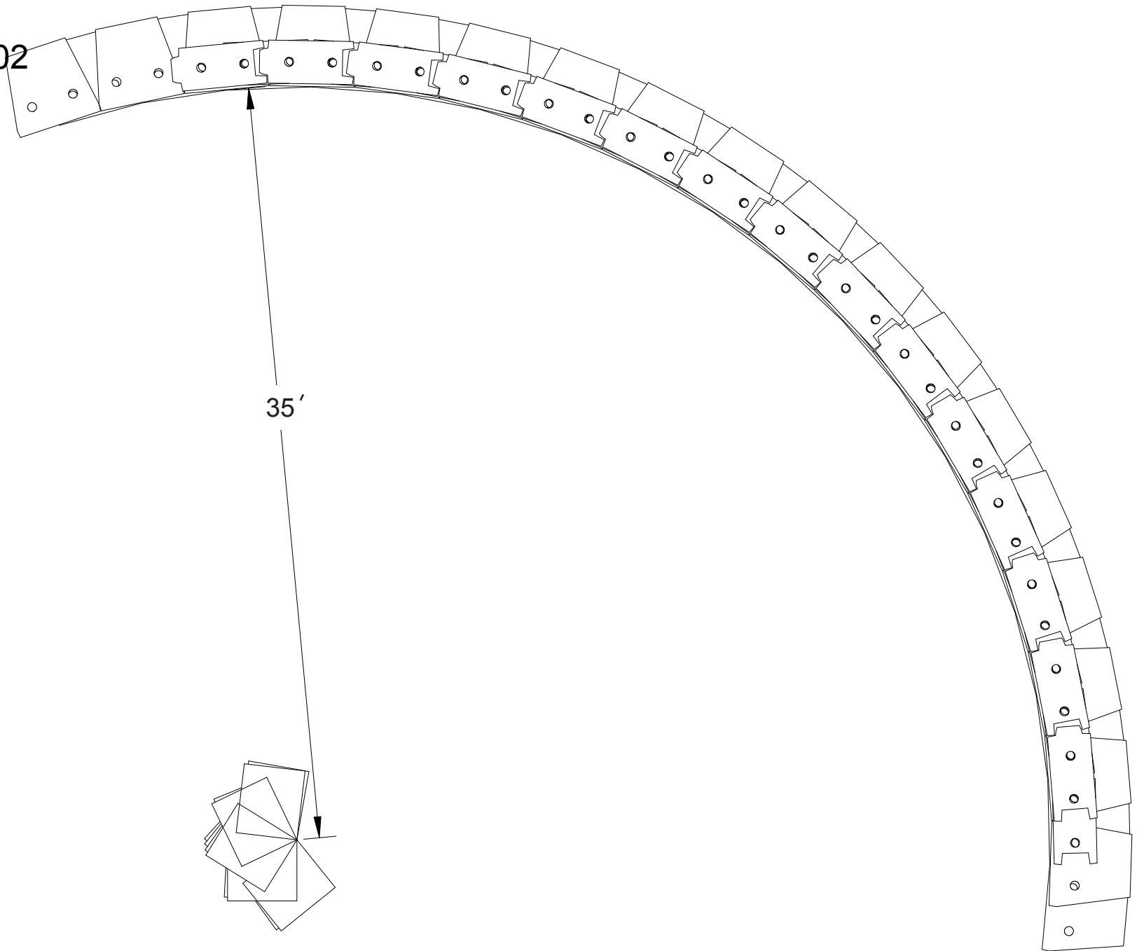
ReCon Guardrail Block Minimum Turning Radius, Inside Curve 35' Radius with .8" spacing left between Guardrail Blocks when placed end to end
